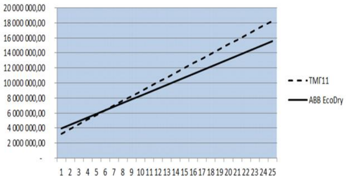
Figure 3. Comparative characteristics of the total cost of two types of traditional (TMГ11) and energy-saving (ABB EcoDry) transformers over the entire service life (25 years).
