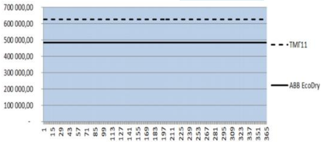
Figure 1 – Comparative characteristics of the cost of electricity losses per year of two types of conventional (TMГ11) and energy-saving (ABB EcoDry) transformers
