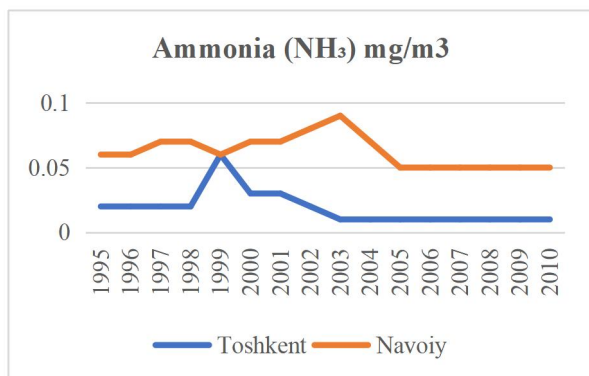
Figure 1. Fluctuation graph of atmospheric pollutant gases in Tashkent and Navoiy cities during 1995–2010.
